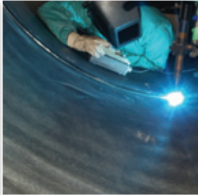
Automated GMAW of Clad Nickel Alloy for duplex reactor
